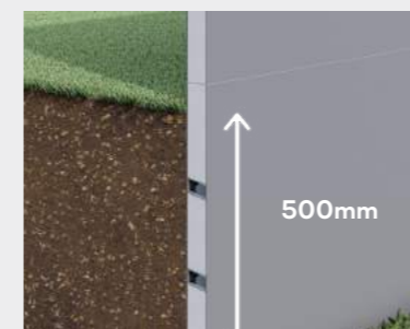
Integrate TerraFirm50 panel (50mm) to retain up to 500mm (2.5 kPa)
